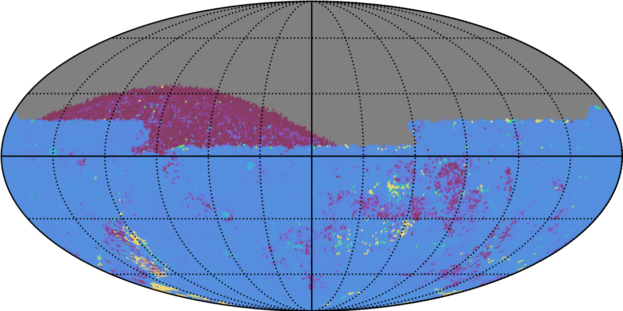
early_u_fpextra4.0_v3.4_10yrs All sky ug bands: 75th Percentile Intranight Timespan
