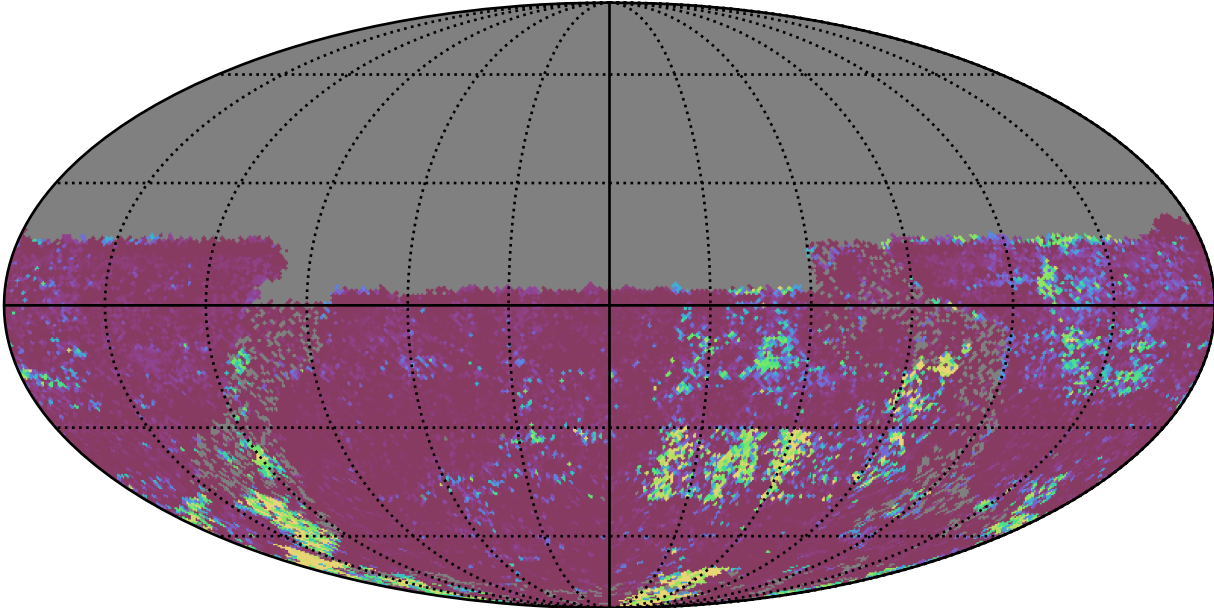
early_u_fpextra4.0_v3.4_10yrs All sky u band: 75th Percentile Intranight Timespan
