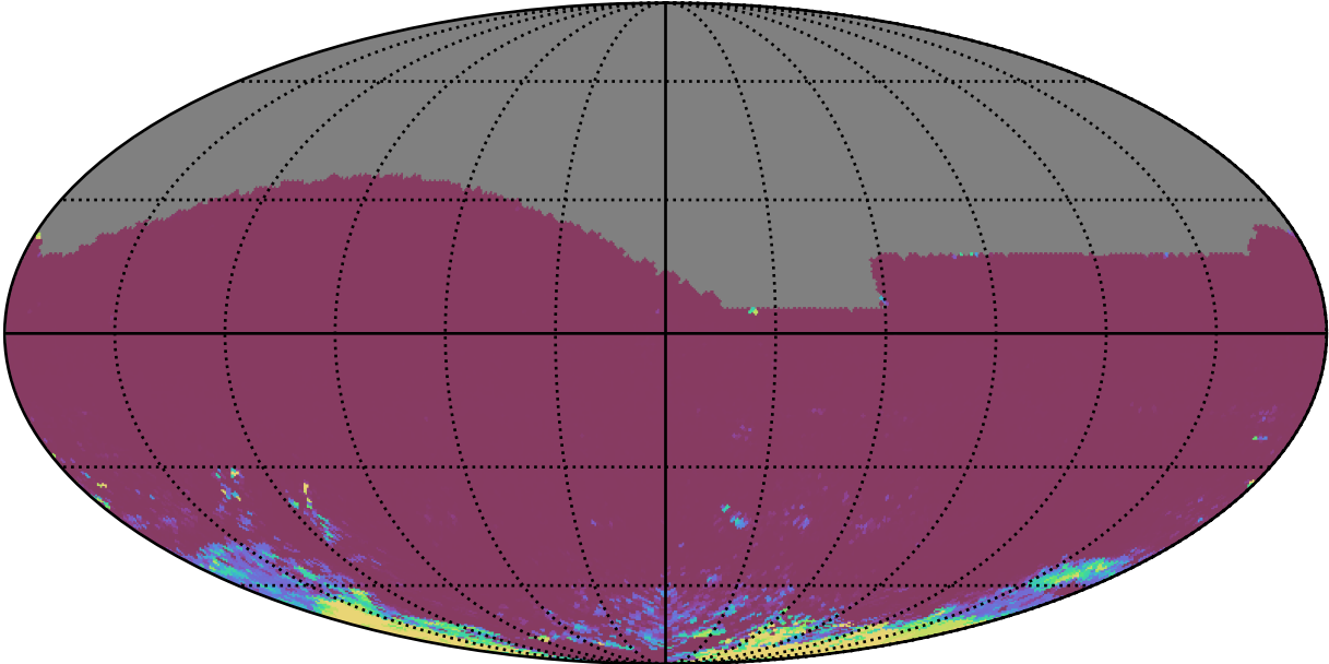
early_u_fpextra4.0_v3.4_10yrs All sky ri bands: 75th Percentile Intranight Timespan
