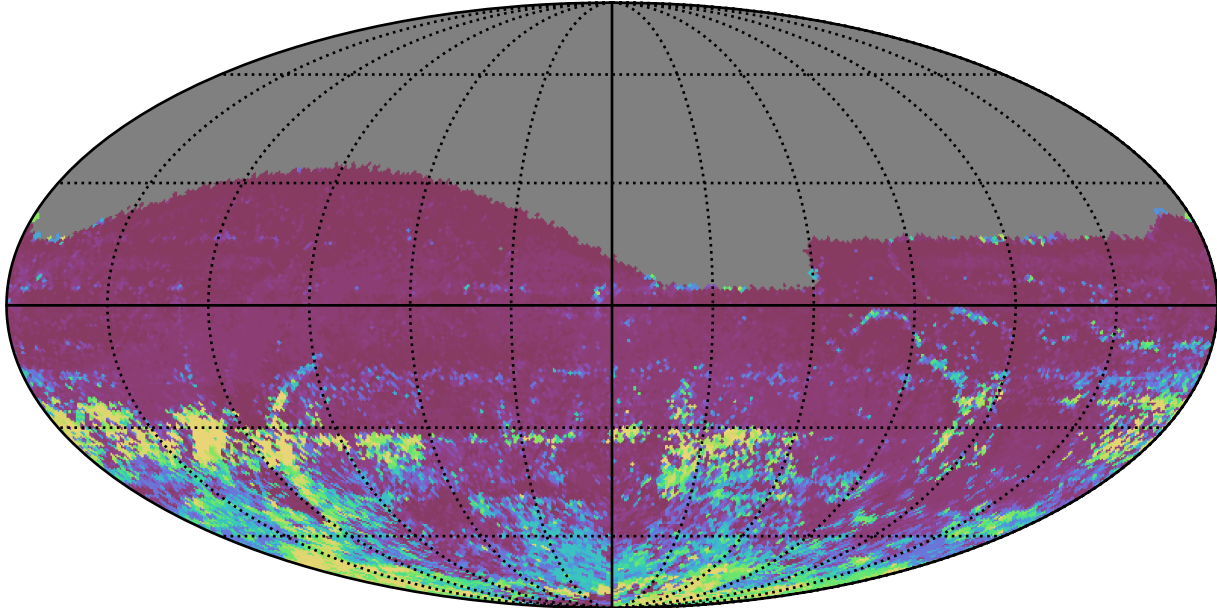
early_u_fpextra4.0_v3.4_10yrs All sky r band: 75th Percentile Intranight Timespan
