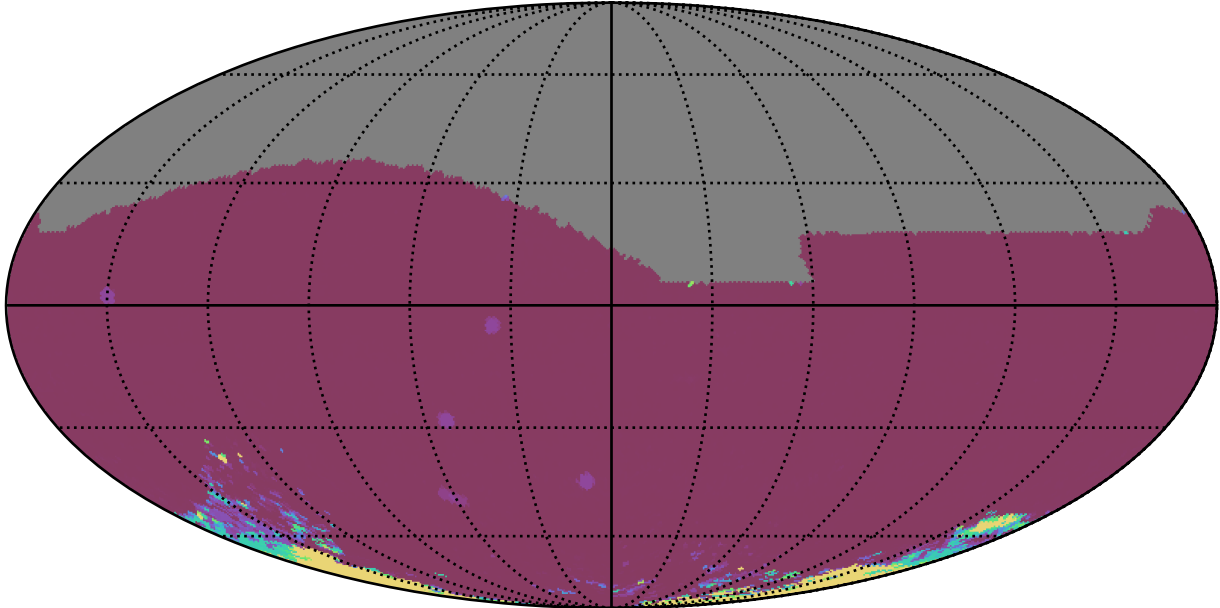
early_u_fpextra4.0_v3.4_10yrs All sky iz bands: 75th Percentile Intranight Timespan
