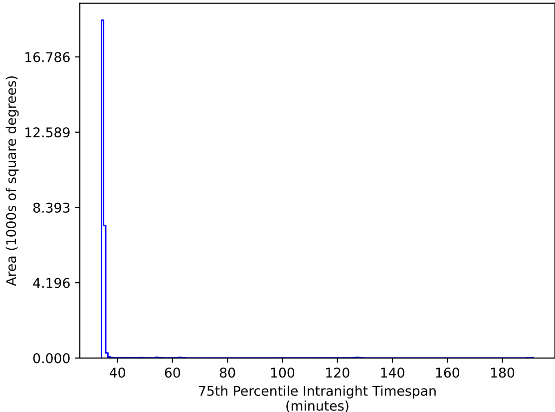
early_u_fpextra4.0_v3.4_10yrs All sky iz bands: 75th Percentile Intranight Timespan
