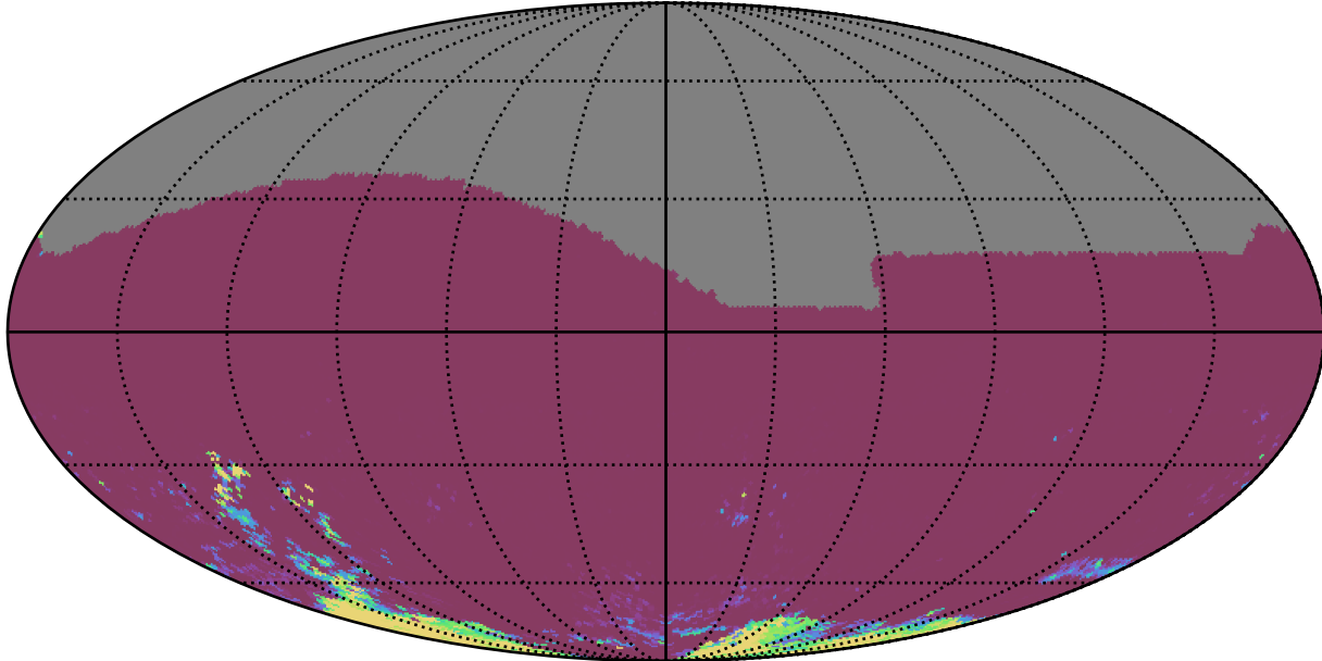
early_u_fpextra4.0_v3.4_10yrs All sky gr bands: 75th Percentile Intranight Timespan
