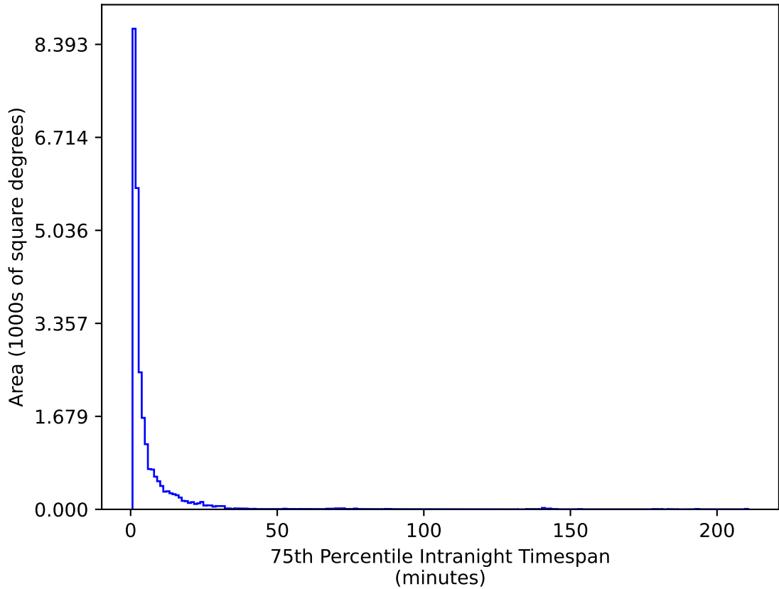
early_u_fpextra4.0_v3.4_10yrs All sky g band: 75th Percentile Intranight Timespan
