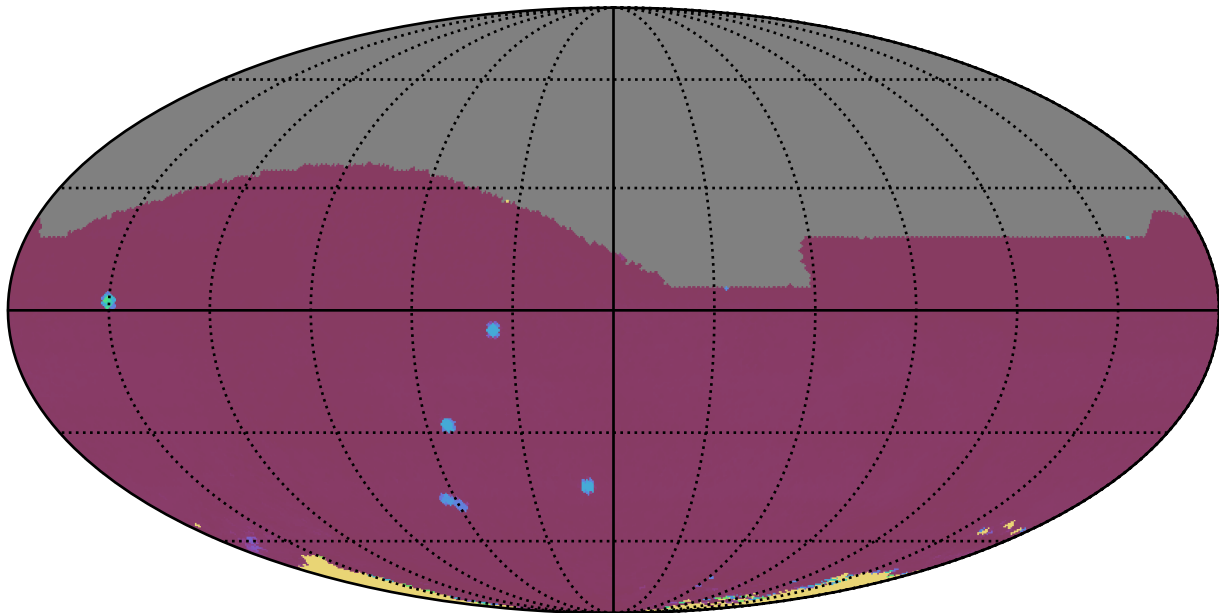
early_u_fpextra4.0_v3.4_10yrs All sky all bands: 75th Percentile Intranight Timespan
