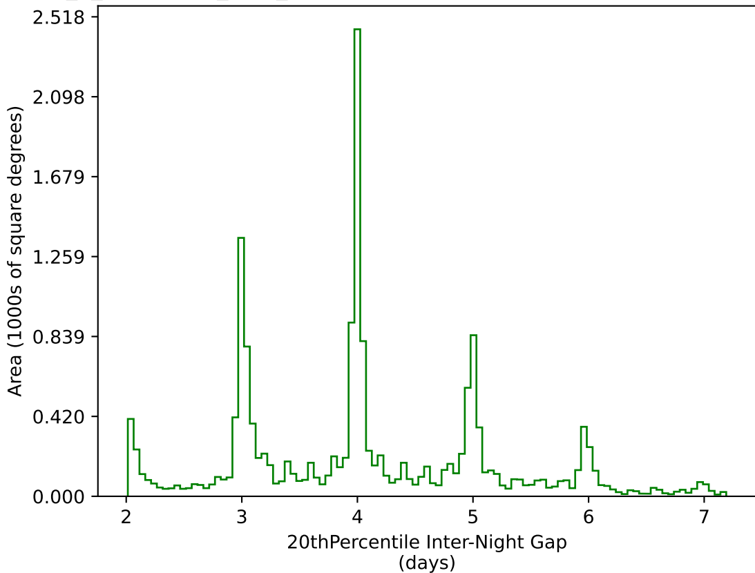
early_u_fpextra4.0_v3.4_10yrs WFD g band: 20thPercentile Inter-Night Gap
