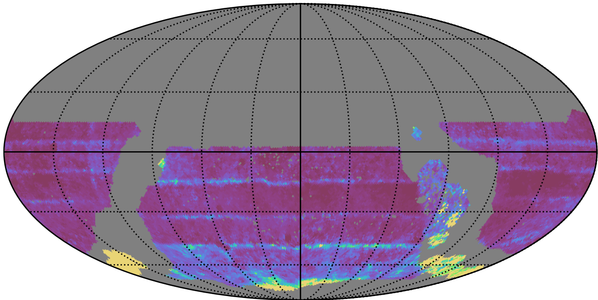
early_u_fpextra4.0_v3.4_10yrs WFD all bands: 20thPercentile Inter-Night Gap
