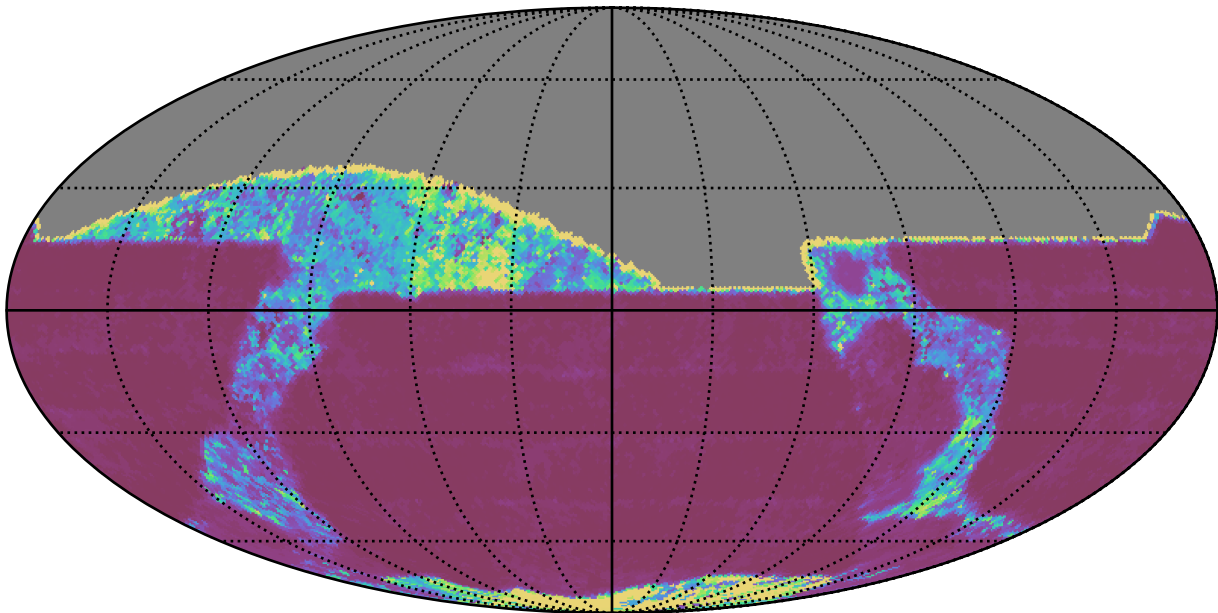
early_u_fpextra4.0_v3.4_10yrs All sky z band: 20thPercentile Inter-Night Gap
