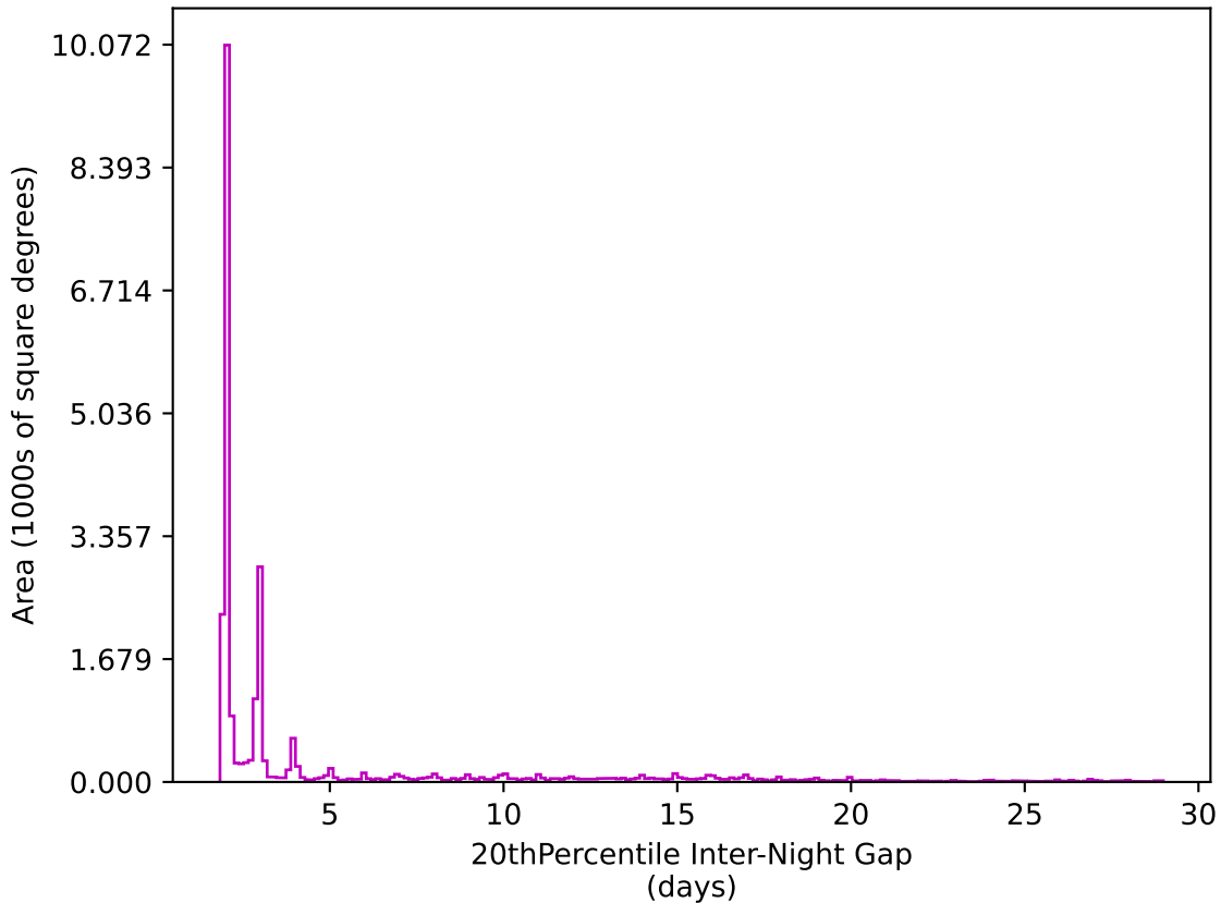
early_u_fpextra4.0_v3.4_10yrs All sky z band: 20thPercentile Inter-Night Gap
