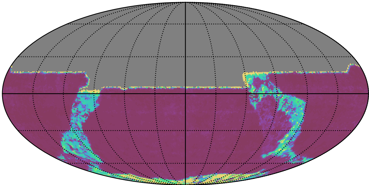
early_u_fpextra4.0_v3.4_10yrs All sky y band: 20thPercentile Inter-Night Gap
