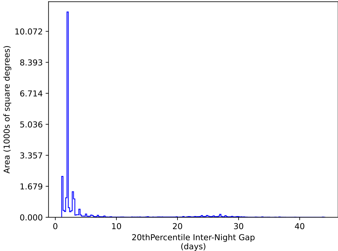
early_u_fpextra4.0_v3.4_10yrs All sky y band: 20thPercentile Inter-Night Gap
