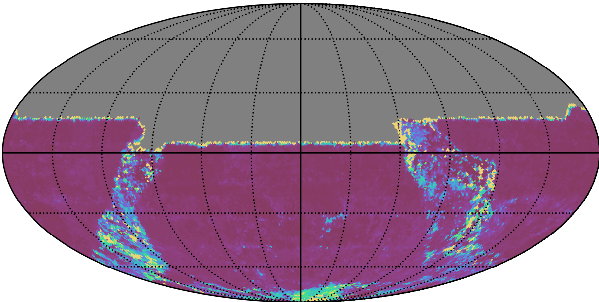
early_u_fpextra4.0_v3.4_10yrs All sky u band: 20thPercentile Inter-Night Gap
