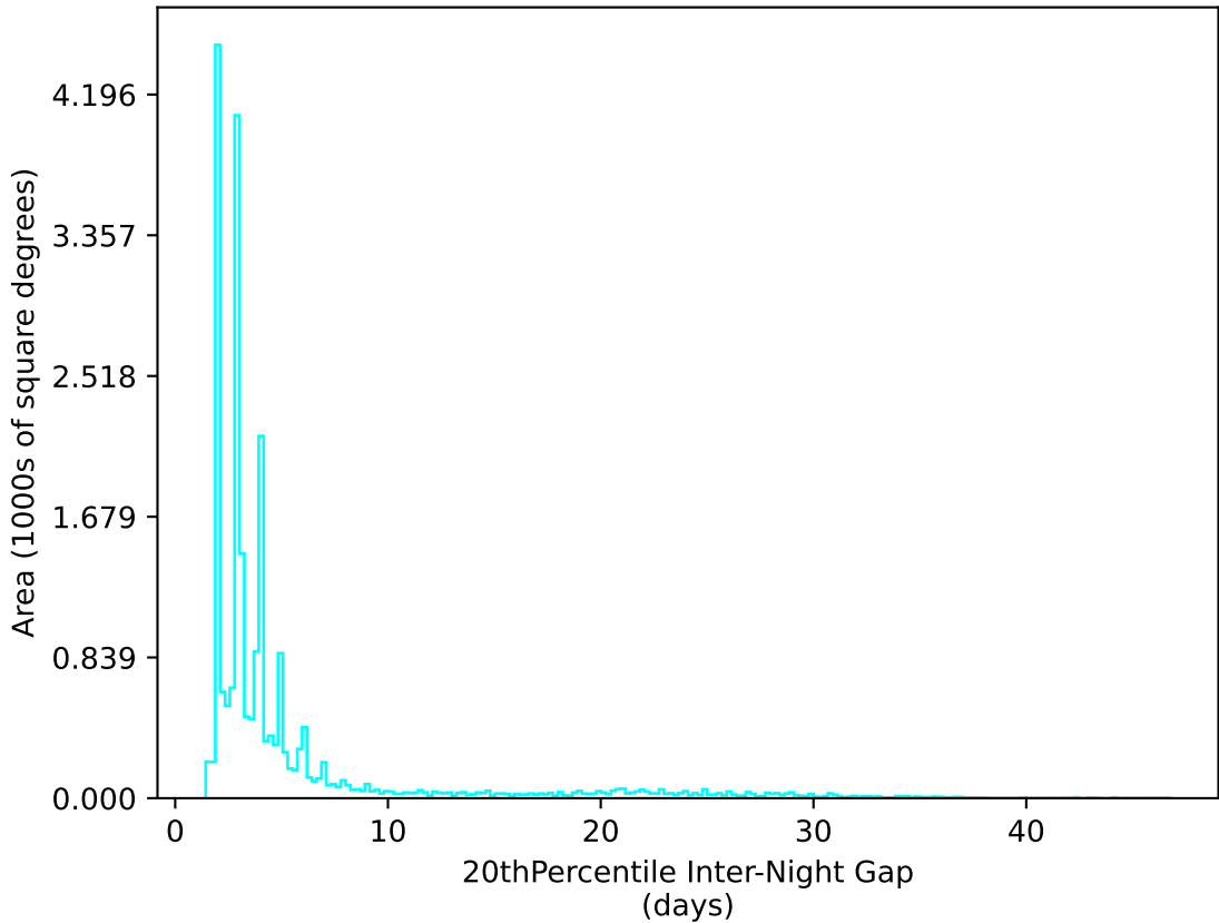
early_u_fpextra4.0_v3.4_10yrs All sky u band: 20thPercentile Inter-Night Gap
