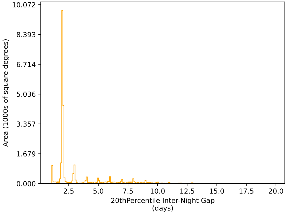
early_u_fpextra4.0_v3.4_10yrs All sky r band: 20thPercentile Inter-Night Gap
