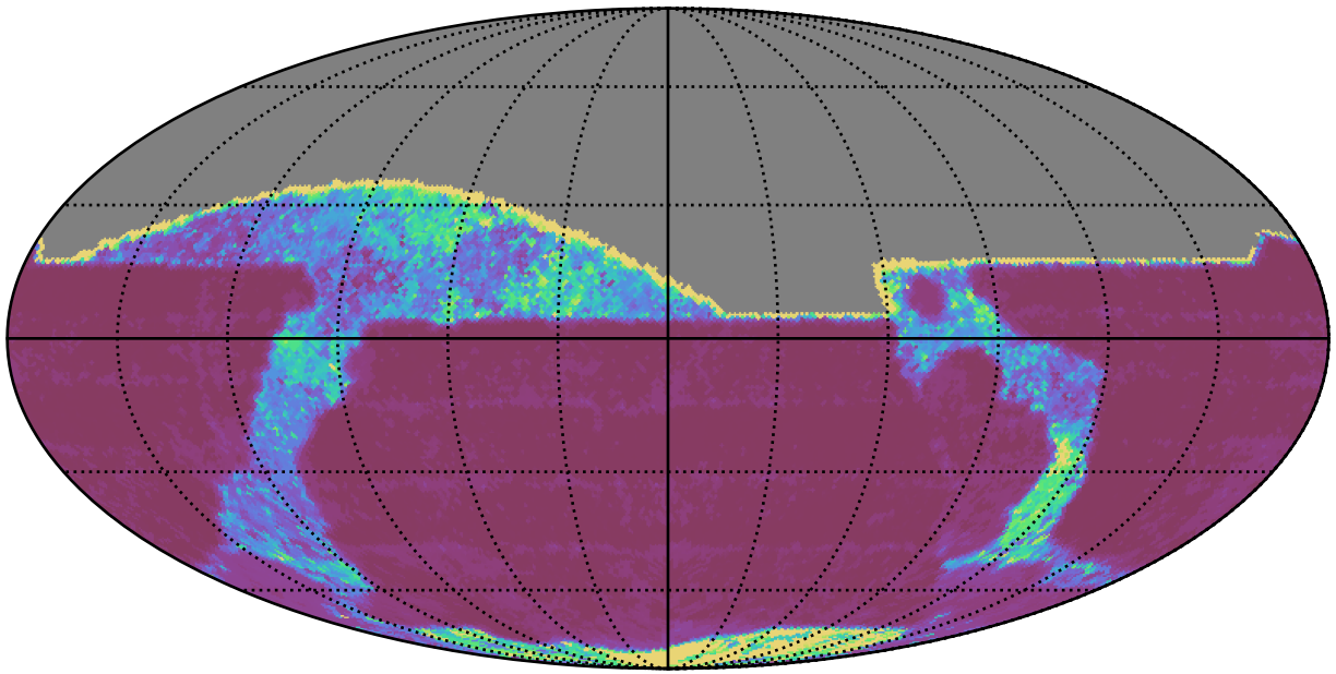
early_u_fpextra4.0_v3.4_10yrs All sky i band: 20thPercentile Inter-Night Gap
