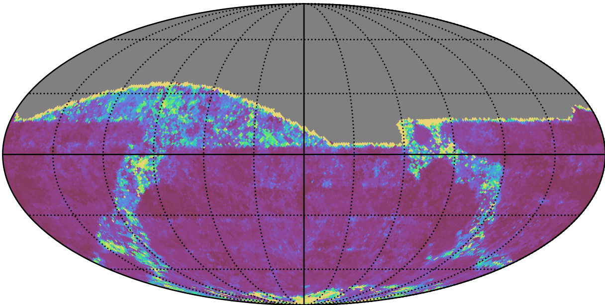
early_u_fpextra4.0_v3.4_10yrs All sky g band: 20thPercentile Inter-Night Gap
