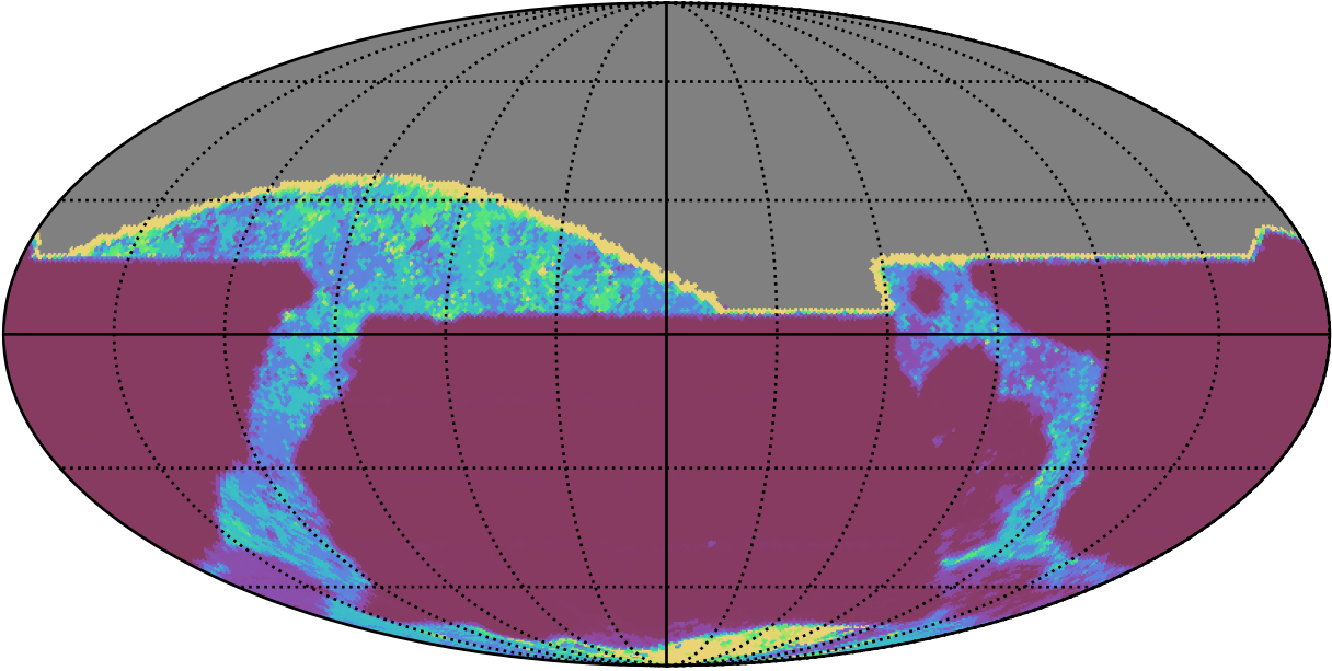
early_u_fpextra4.0_v3.4_10yrs All sky all bands: 20thPercentile Inter-Night Gap
