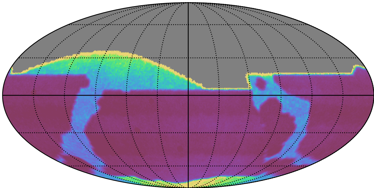
early_u_fpextra4.0_v3.4_10yrs : properMotion
