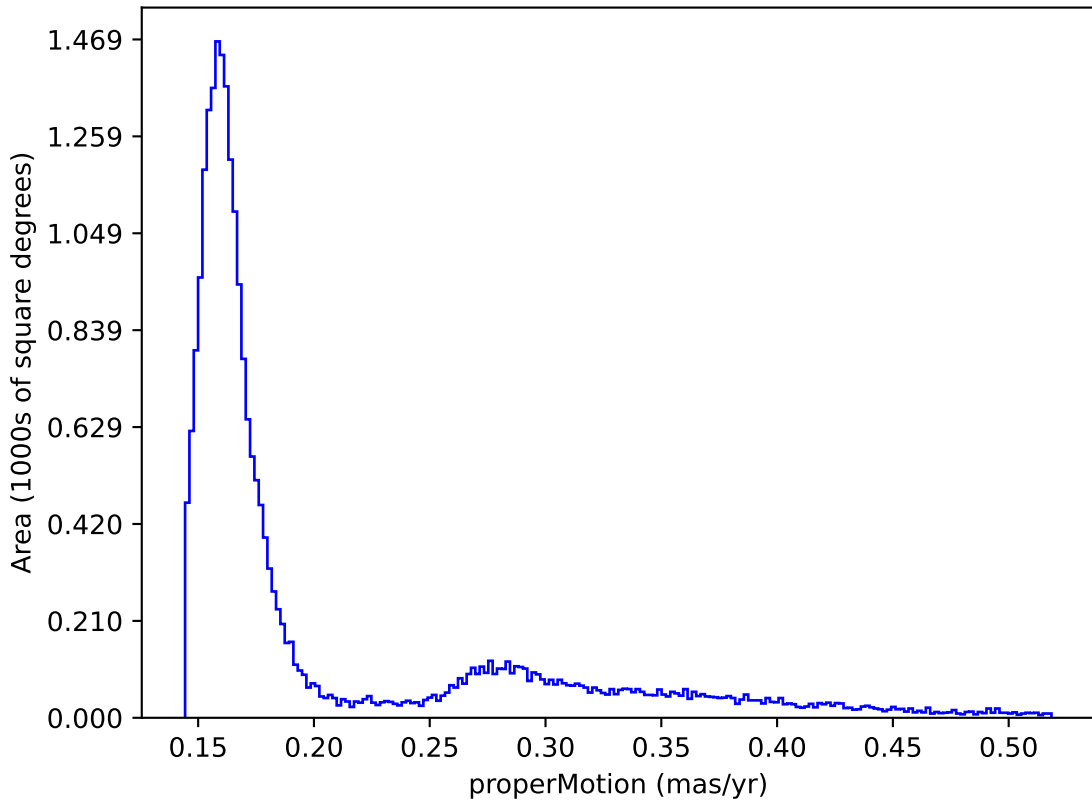
early_u_fpextra4.0_v3.4_10yrs : properMotion
