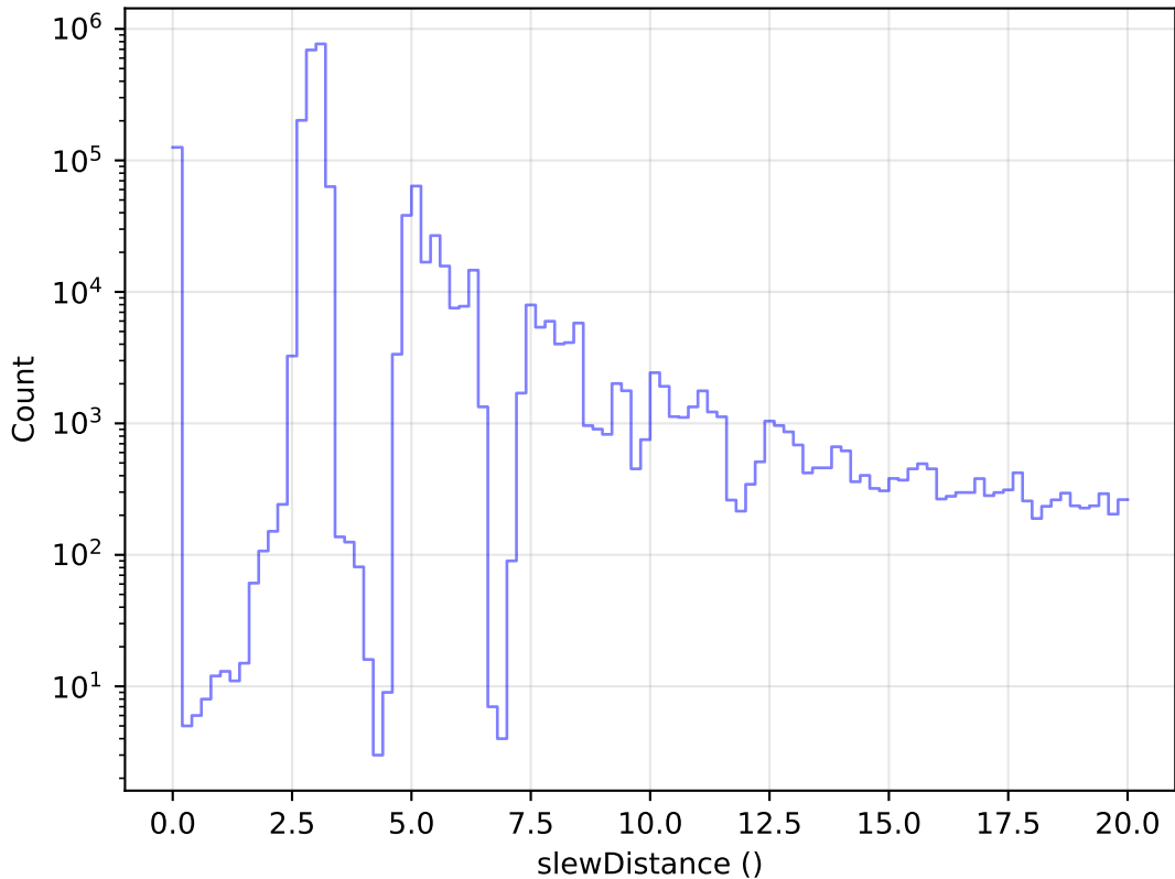
early_u_fpextra4.0_v3.4_10yrs All visits: Zoom Slew Distance Histogram
