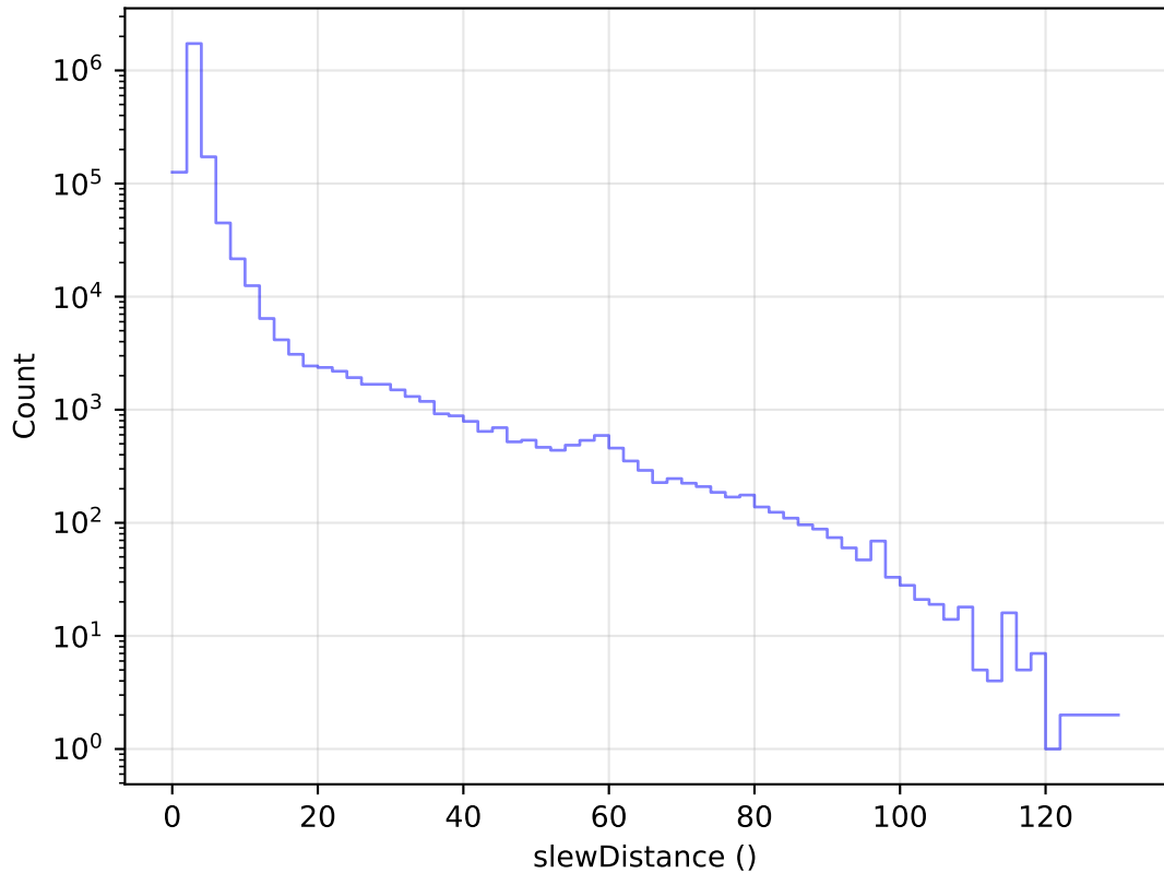
early_u_fpextra4.0_v3.4_10yrs All visits: Slew Distance Histogram
