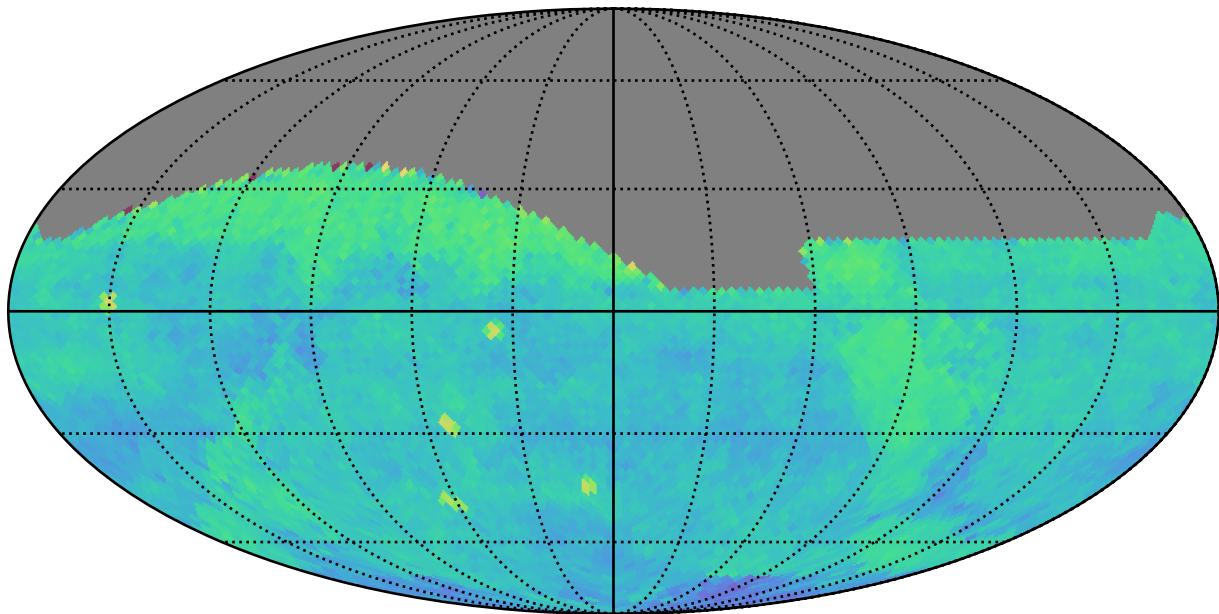
early_u_fpextra4.0_v3.4_10yrs (g or r or i): PairFraction
