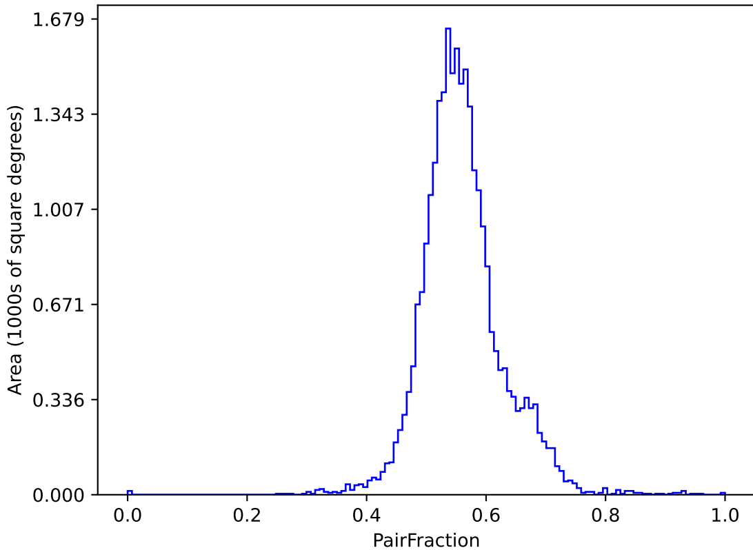
early_u_fpextra4.0_v3.4_10yrs (g or r or i): PairFraction
