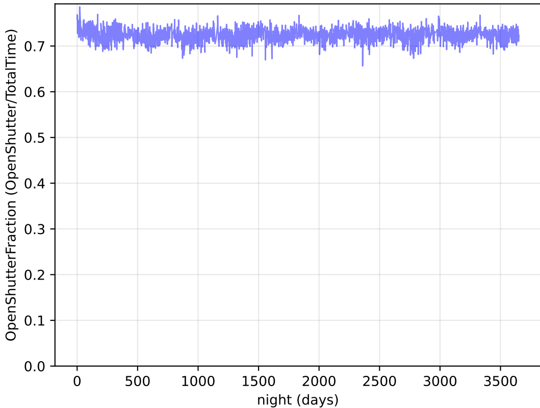
early_u_fpextra4.0_v3.4_10yrs : OpenShutterFraction
