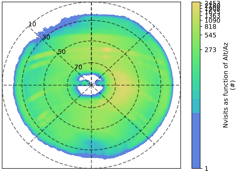
early_u_fpextra4.0_v3.4_10yrs z: Nvisits as function of Alt/Az
