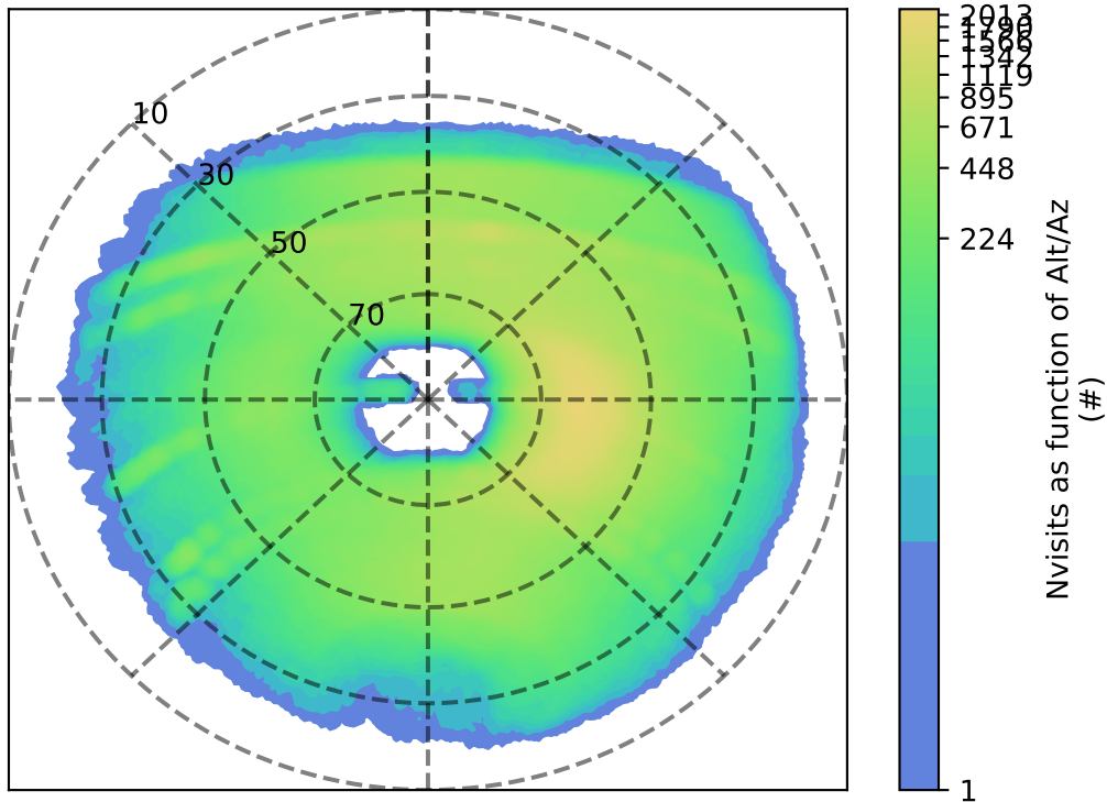
early_u_fpextra4.0_v3.4_10yrs y: Nvisits as function of Alt/Az
