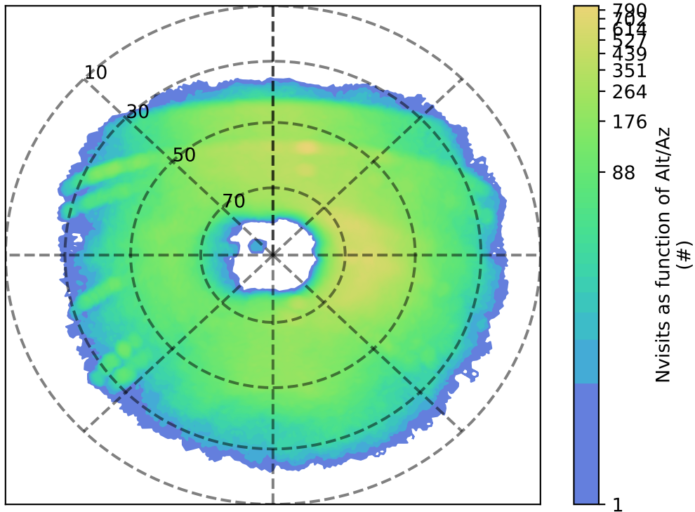
early_u_fpextra4.0_v3.4_10yrs u: Nvisits as function of Alt/Az
