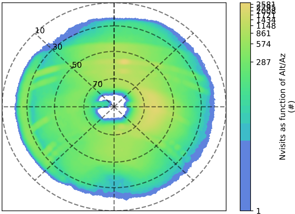
early_u_fpextra4.0_v3.4_10yrs r: Nvisits as function of Alt/Az
