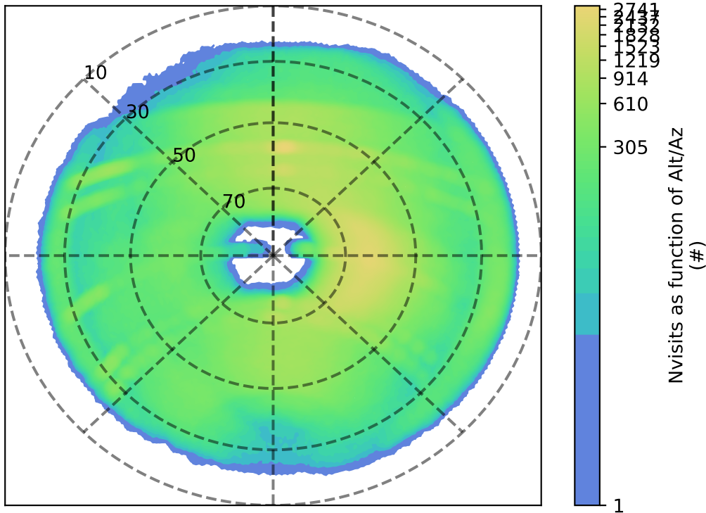
early_u_fpextra4.0_v3.4_10yrs i: Nvisits as function of Alt/Az
