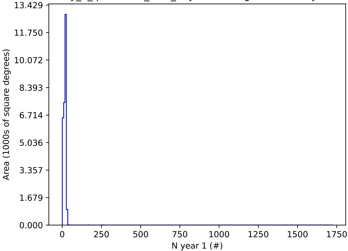
early_u_fpextra4.0_v3.4_10yrs i and night < 365: N year 1
