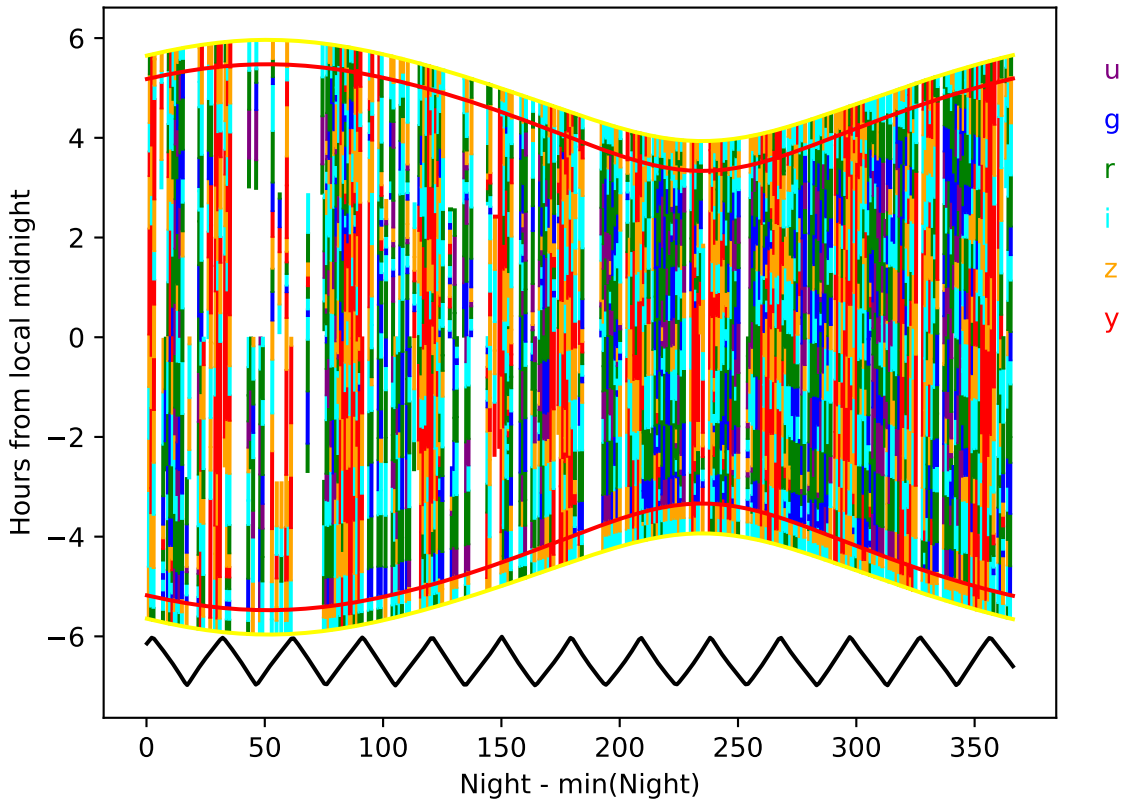
early_u_fpextra4.0_v3.4_10yrs year 9-10: Hourglass
