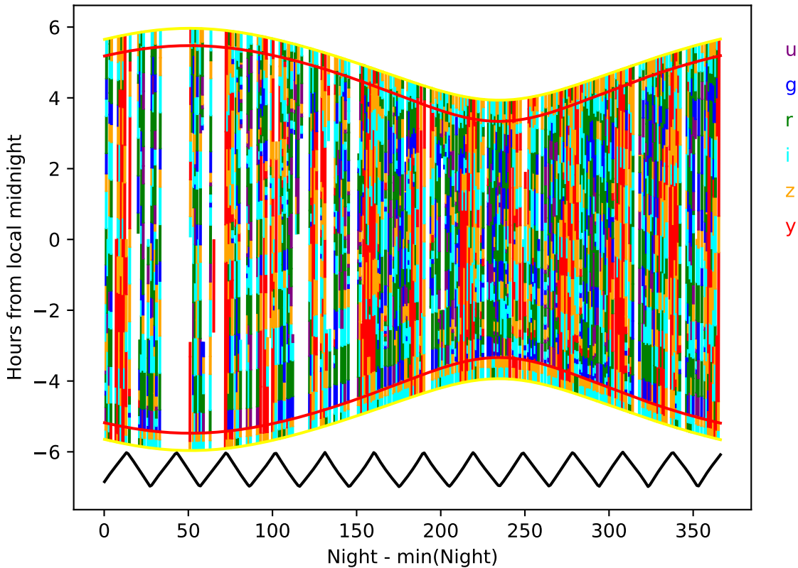
early_u_fpextra4.0_v3.4_10yrs year 8-9: Hourglass
