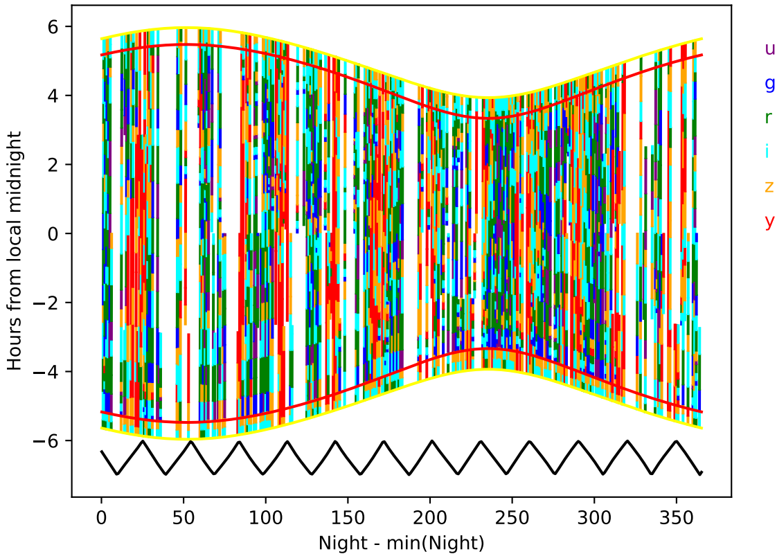
early_u_fpextra4.0_v3.4_10yrs year 7-8: Hourglass
