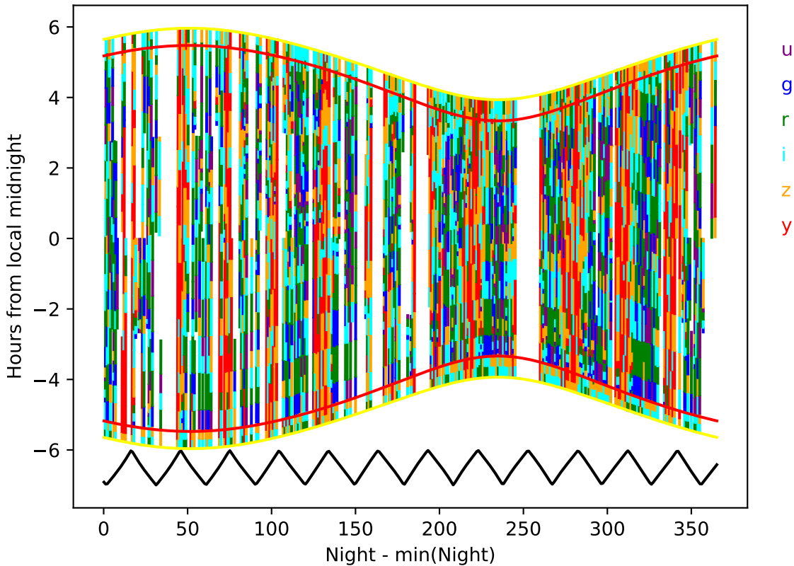
early_u_fpextra4.0_v3.4_10yrs year 5-6: Hourglass
