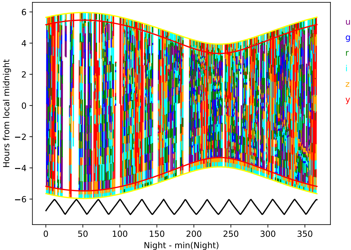
early_u_fpextra4.0_v3.4_10yrs year 0-1: Hourglass
