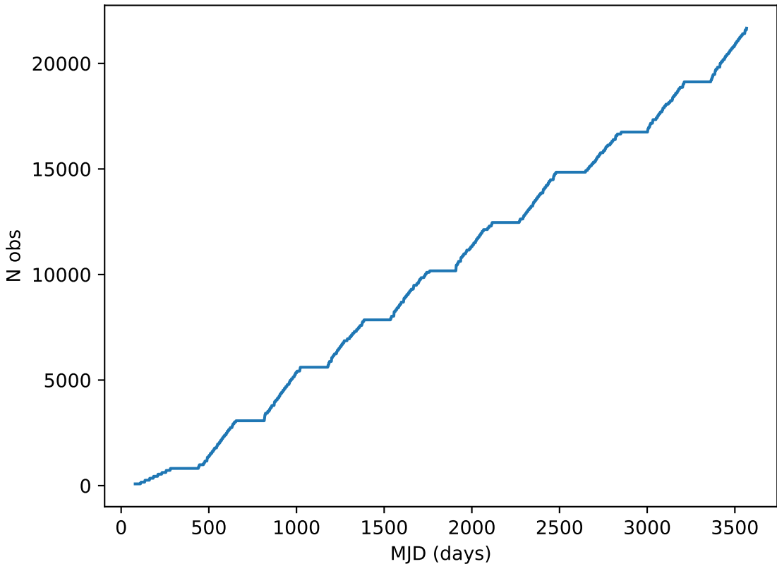
early_u_fpextra4.0_v3.4_10yrs note like DD:XMM_LSS%: Cumulative
