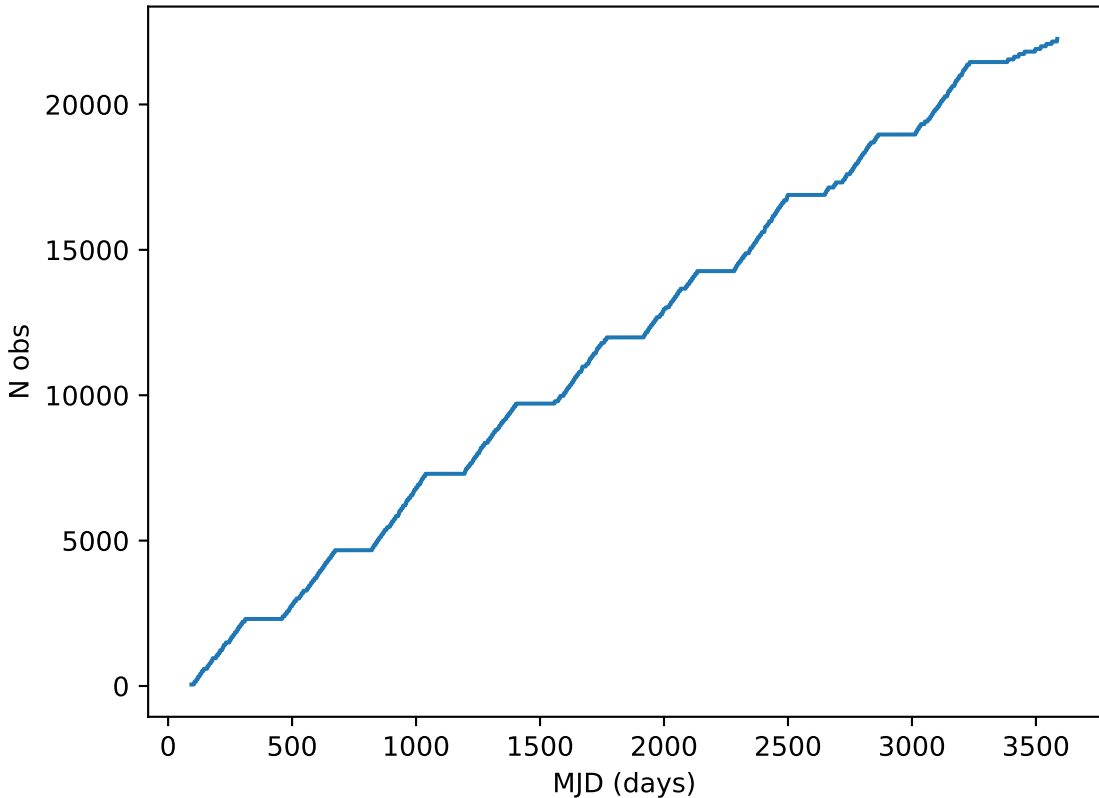
early_u_fpextra4.0_v3.4_10yrs note like DD:ECDFS%: Cumulative
