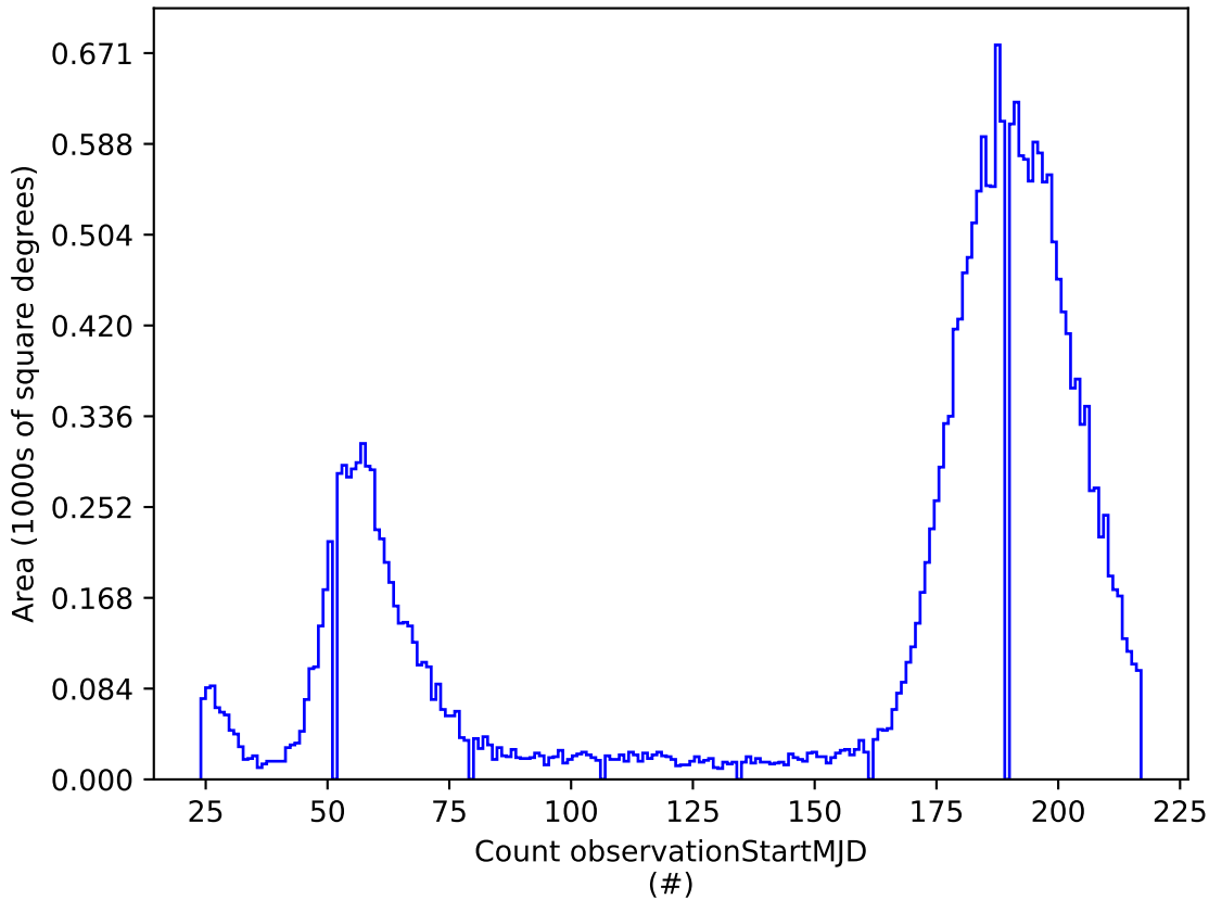
early_u_fpextra4.0_v3.4_10yrs i: Count observationStartMJD
