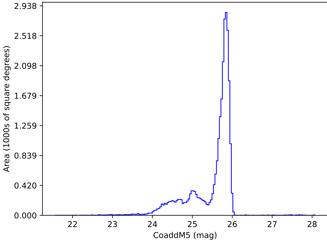
early_u_fpextra4.0_v3.4_10yrs z: CoaddM5
