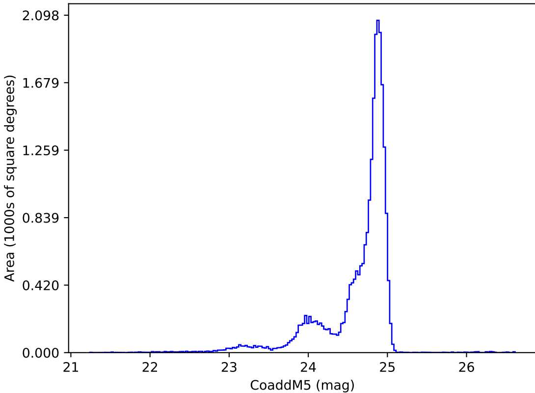
early_u_fpextra4.0_v3.4_10yrs y: CoaddM5
