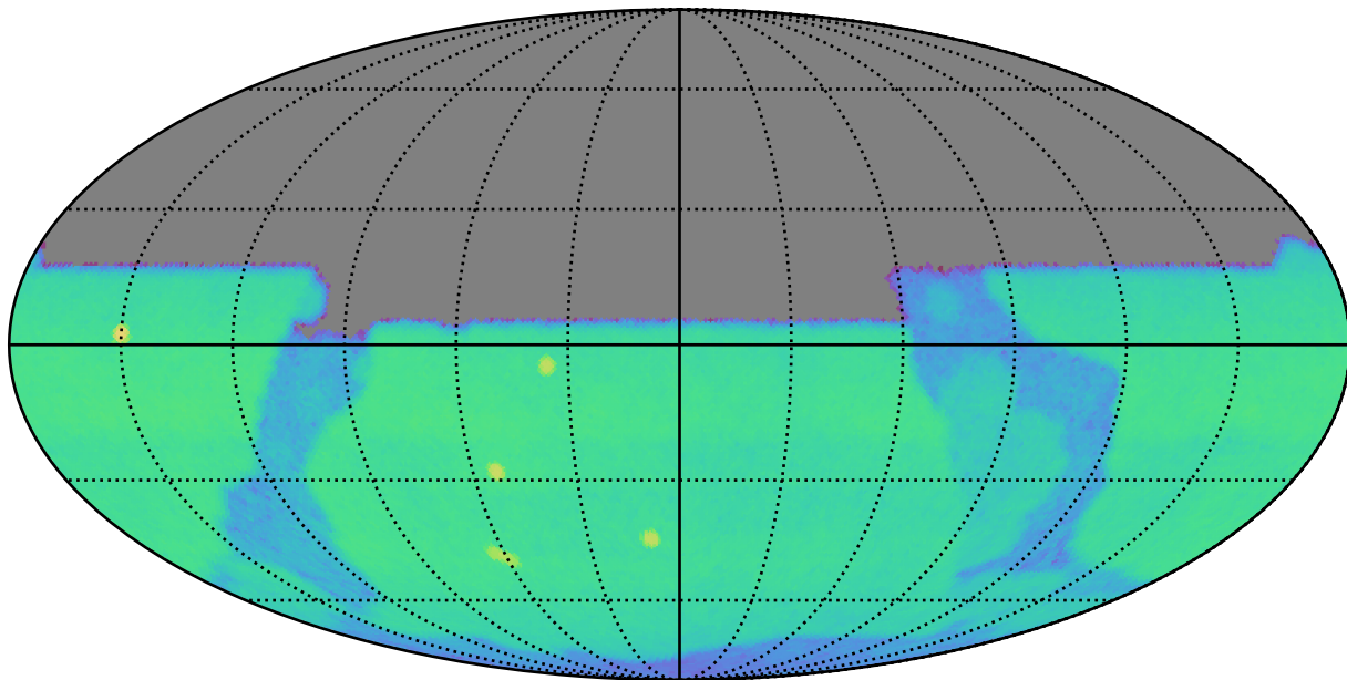
early_u_fpextra4.0_v3.4_10yrs u: CoaddM5
