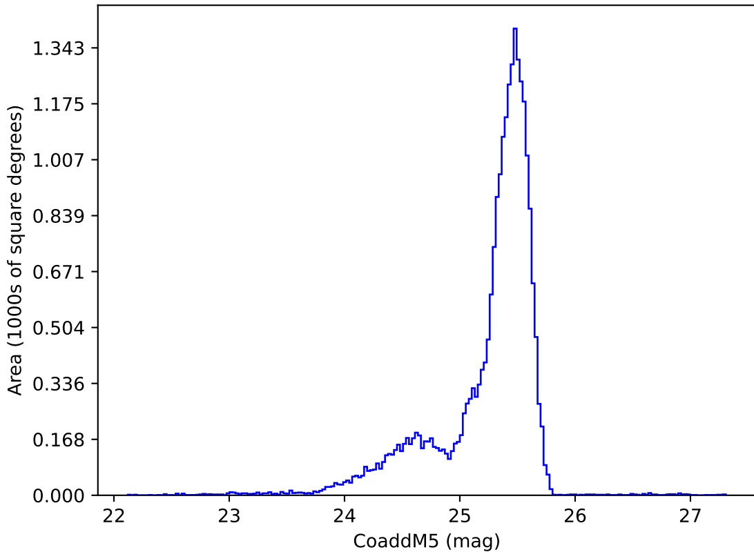
early_u_fpextra4.0_v3.4_10yrs u: CoaddM5
