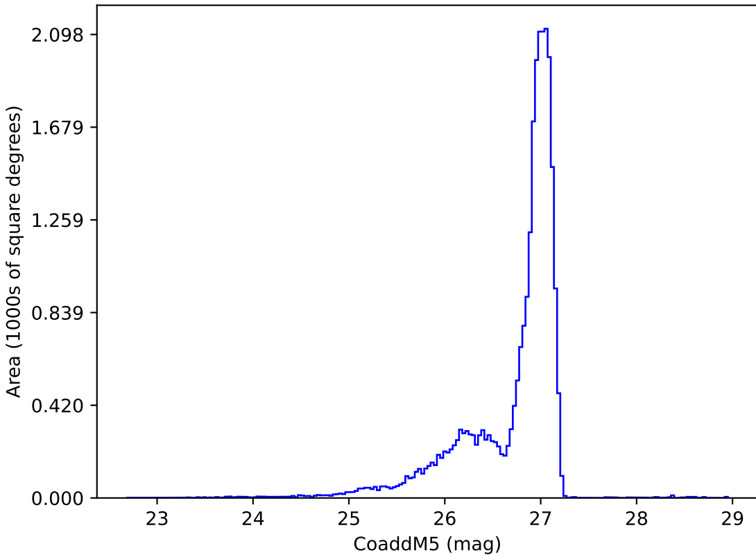
early_u_fpextra4.0_v3.4_10yrs r: CoaddM5
