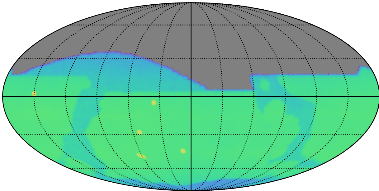
early_u_fpextra4.0_v3.4_10yrs i: CoaddM5
