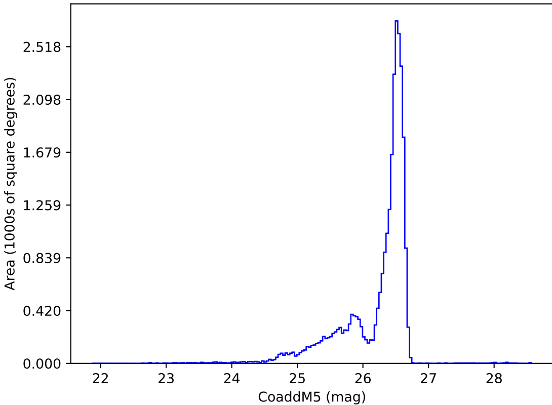
early_u_fpextra4.0_v3.4_10yrs i: CoaddM5
