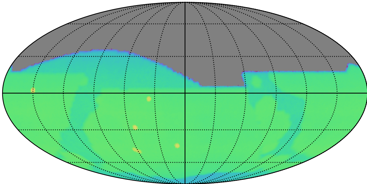
early_u_fpextra4.0_v3.4_10yrs : CoaddM5
